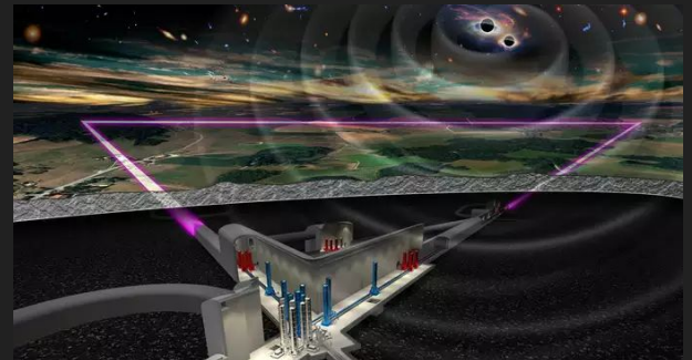
Artist illustrations of the SKA (credit: SKAO) and ET (credit NIKHEF).
