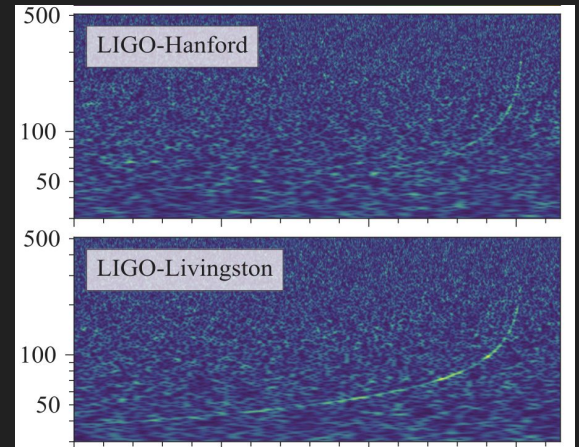
The merger of two NSs (top illustration by NASA Goddard) produces a characteristic chirp signal (bottom) in a gravitational wave detector (Abbott et al., 2017).
