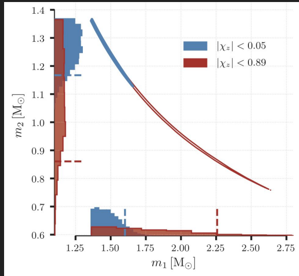
Mass posteriors for the component masses of GW170817 (Abbott et al., 2017).
