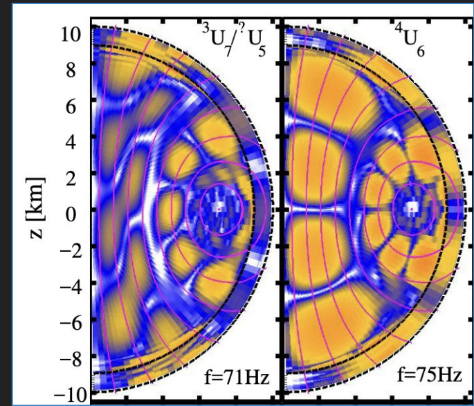
Amplitude of discrete Fourier transform of velocity field of strongest QPOs (Gabler et al. 2016).
