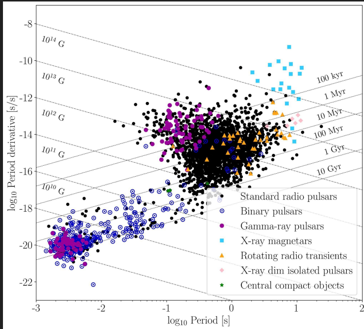
Period period-derivative diagram of the pulsar population. Data taken from ATNF Pulsar Catalogue (Manchester et al. 2005).
