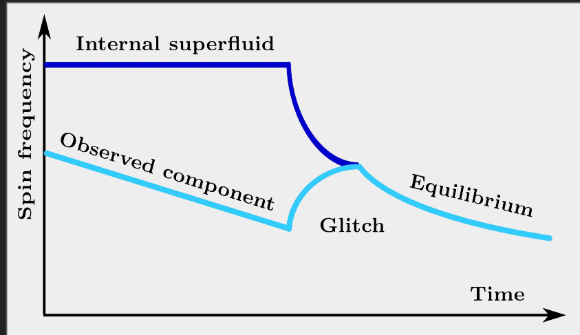
Sketch of the two-component pulsar glitch model.
