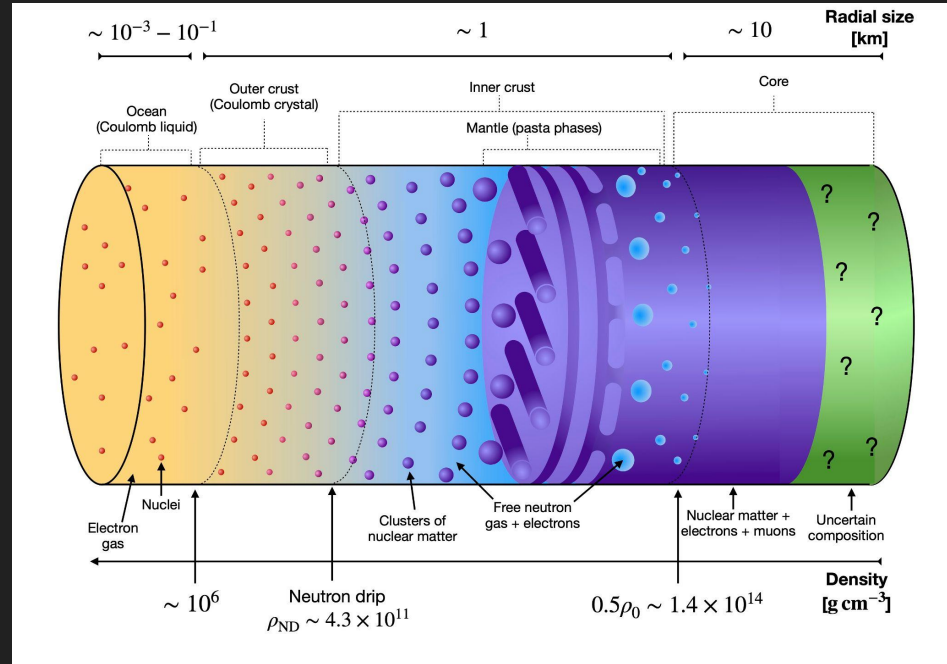
Sketch of the NS structure (Ascenzi, Graber & Rea, 2024).
