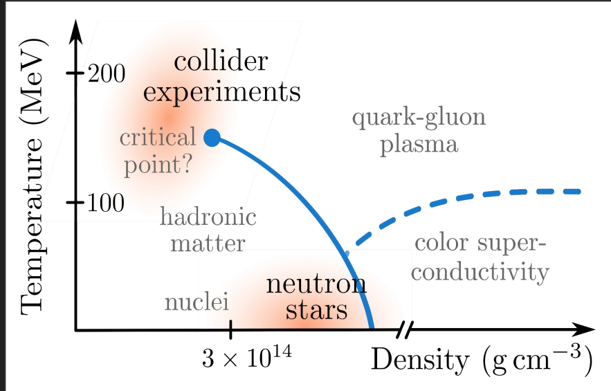
Sketch of the QCD phase diagram showing the complementary regions probed by terrestrial collider experiments and NSs.
